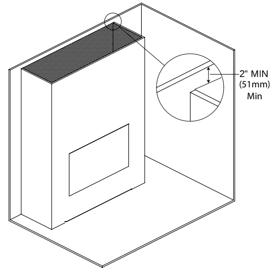
Figure 6: Open Chase - Iso View
