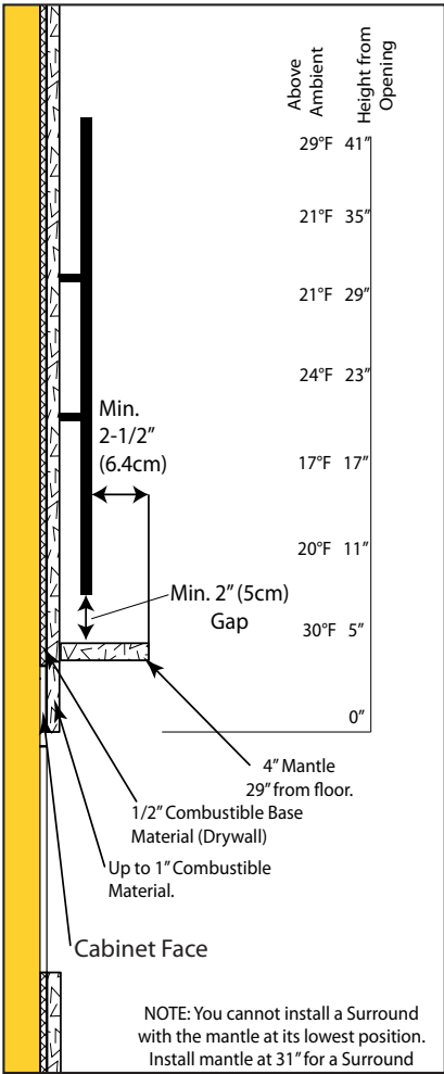
Figure 11: CSS TV - Mantle
