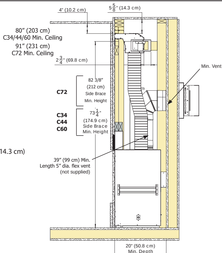
Figure 8: C34 CSS Front Vent Kit - Min. Install
