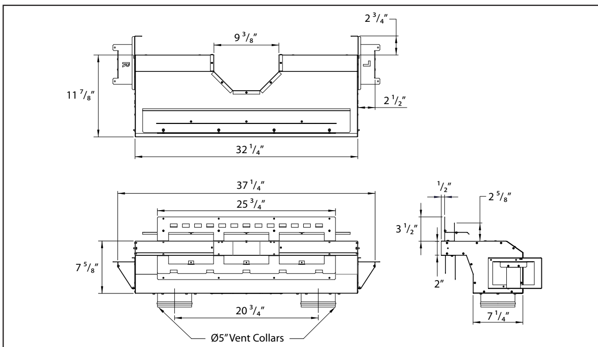
Figure 7: C34 CSS Front Vent Kit - Dimensions
