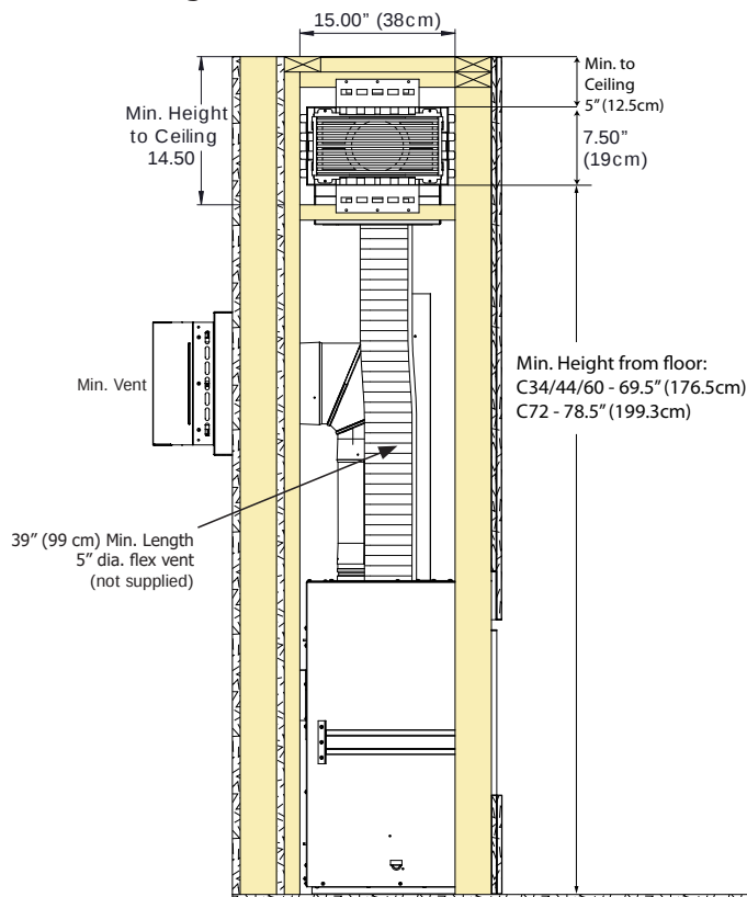
Figure 9: C34 CSS Side Vent Kit - Min. Install
