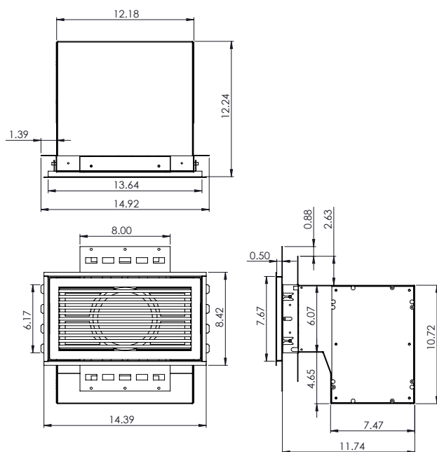
Figure 8: C-Series CSS Side Vent Kit - Dimensions
