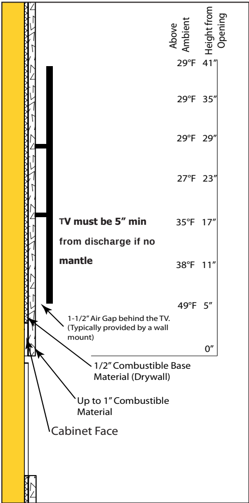
Figure 10: CSS TV - Flat Wall
