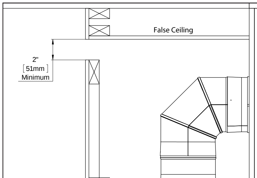
Figure 3: False Ceiling
